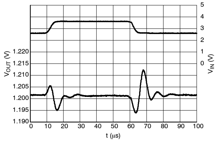
Figure 26. Line Transients, 1.2 V Version, t_R = t_F = 5 \mu s , I_{OUT} = 30 \text{ mA}
